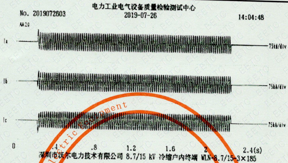
C.6 The waveform of dynamic short-circuit tests of the combination samples
