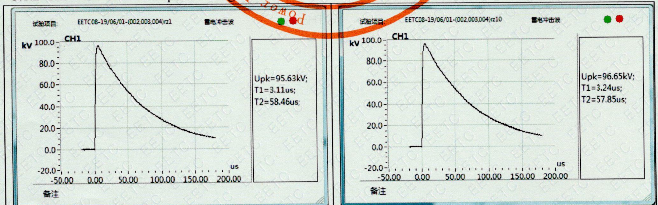
The 10 th positive impulses waveform
