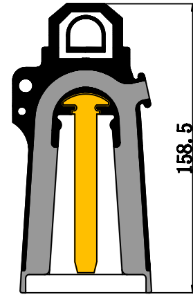
Dimension: mm
