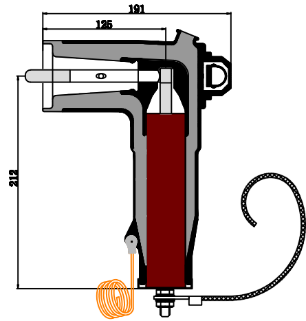
Dimension: mm
