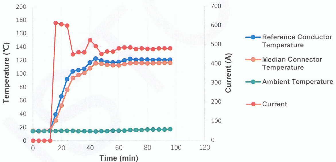
Figure 1 1st heat cycle temperature curve
