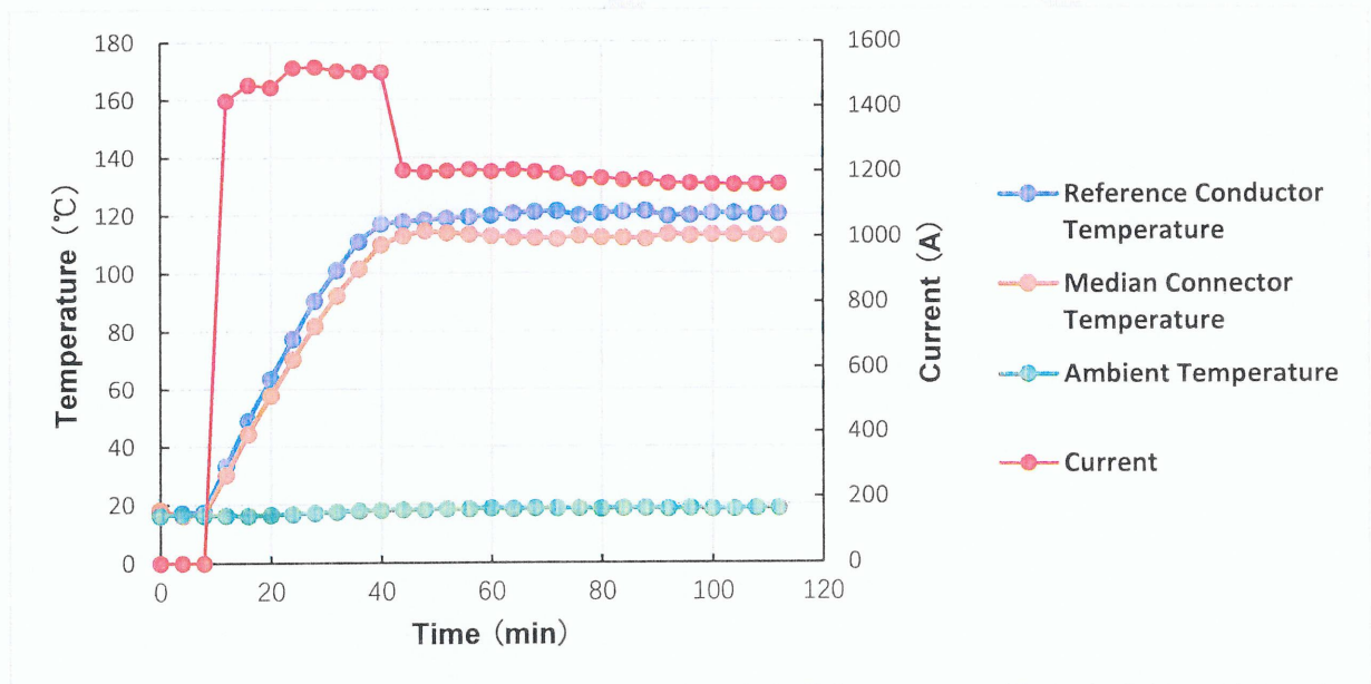
Figure 1 1st heat cycle temperature curve
