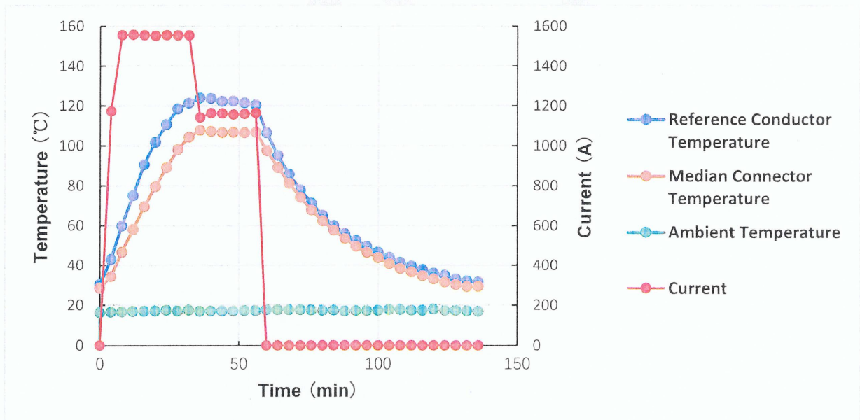
Figure 2 2nd heat cycle temperature curve
